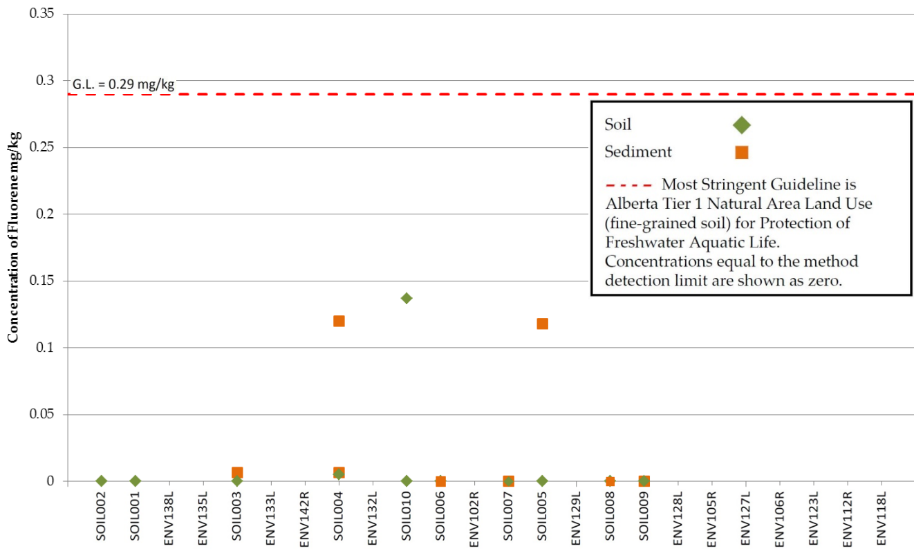
Soil Locations from OBED Mine to 5km Downstream
